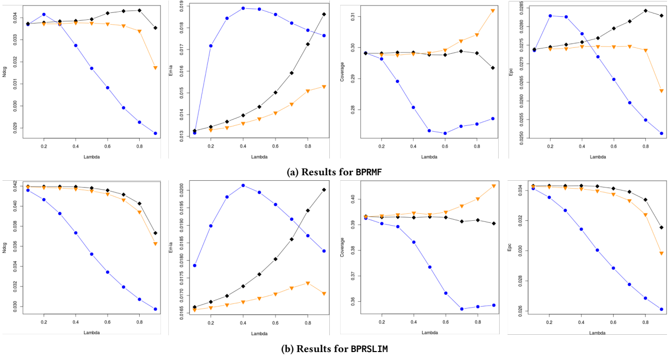
Figure 1: Curves obtained by varying \lambda from 0.1 to 0.9 (step 0.1), using BPRMF and BPRSLIM as recommendation algorithm. From left to right we plot the values of nDCG, ERR-IA, Catalog Coverage and EPC. The blue line represents values for the base xQuAD evaluation while the black and yellow lines represent respectively values for the time-based and session-based version of xQuAD
